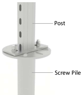
Ground Screw Pile Foundation
